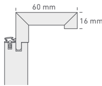
Zarge Eckig 60/16 mm Square architrave
