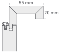
Zarge Eckig 55/20 mm Square architrave
